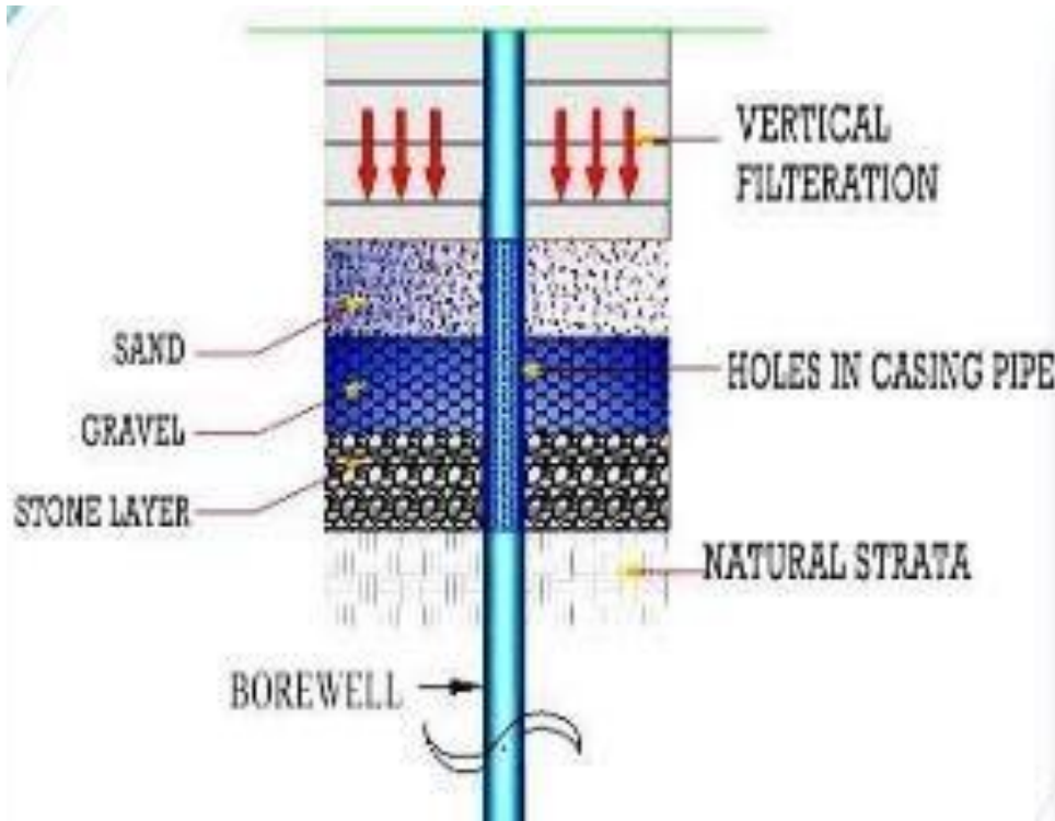
RAIN WATER HARVESTING SYSTEM USING CONVENTIONAL METHOD
