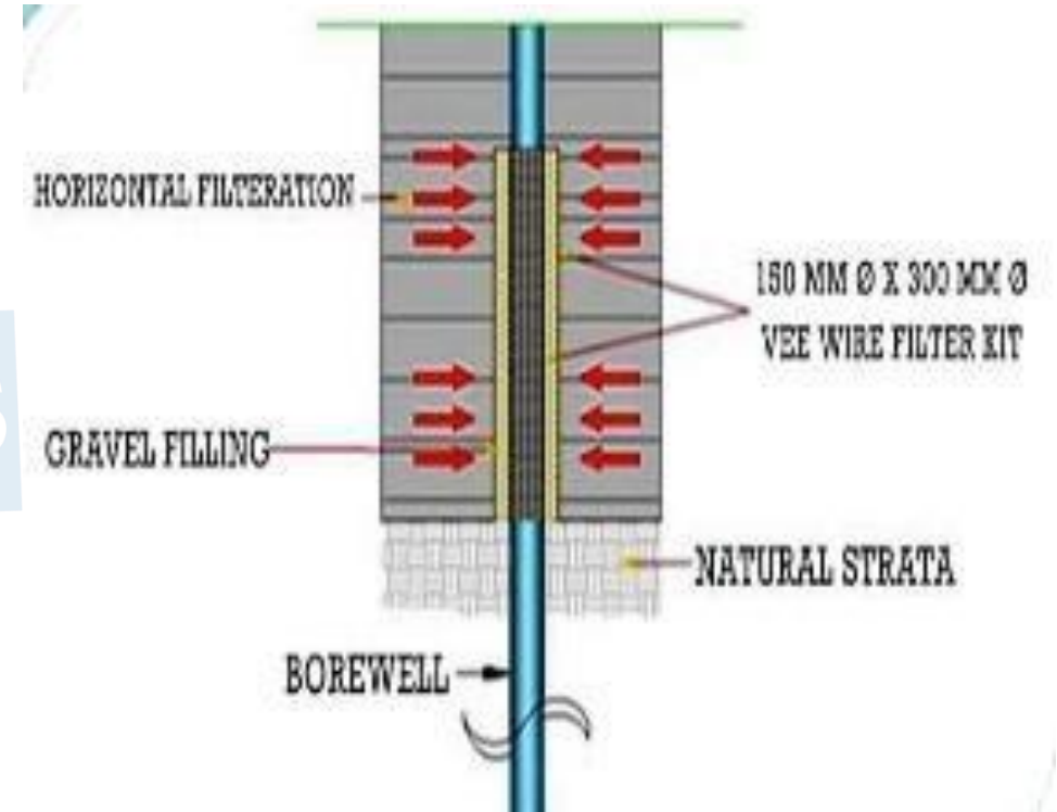
RAIN WATER HARVESTING SYSTEM USING V-WIRE FILTER SCREENS
